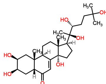
20-hydroxyecdysone (7, (5 \beta )–CHOLESTEN - 2 \beta , 3 \beta , 14 \alpha , 20R, 22R, 25- HEXOL-6-ONE)
